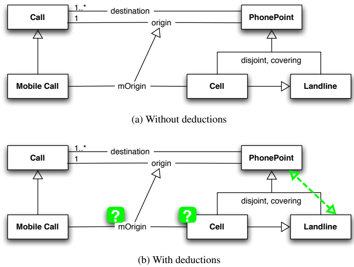
Fig. 2. Second ontology design scenario.
