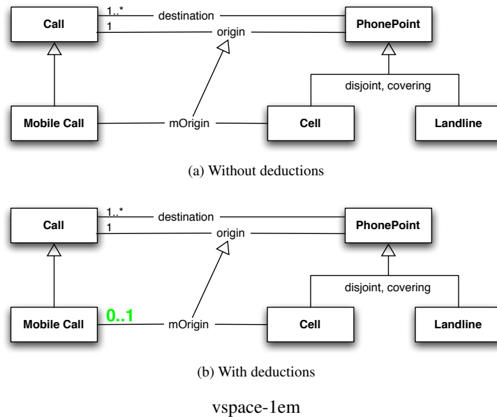
Fig. 1. First ontology design scenario.
